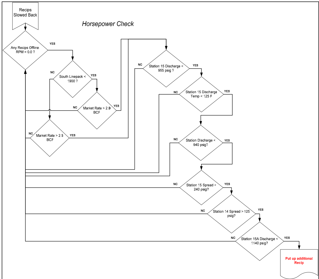
Figure 3. Additional horsepower required alarm
