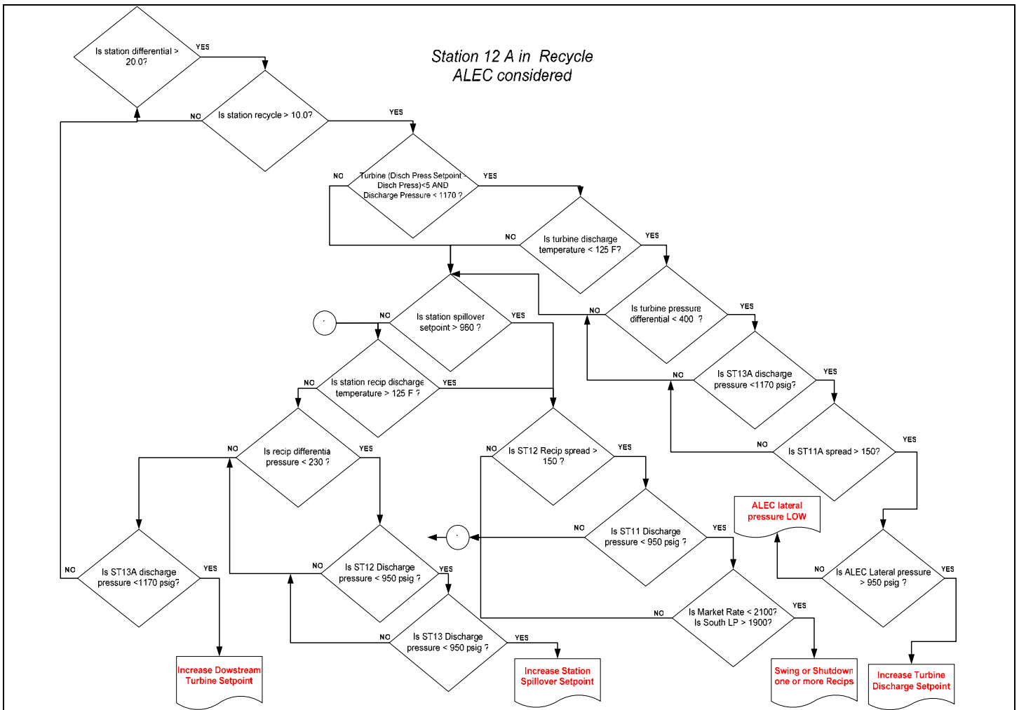
Figure 7. Spillover station alarms
