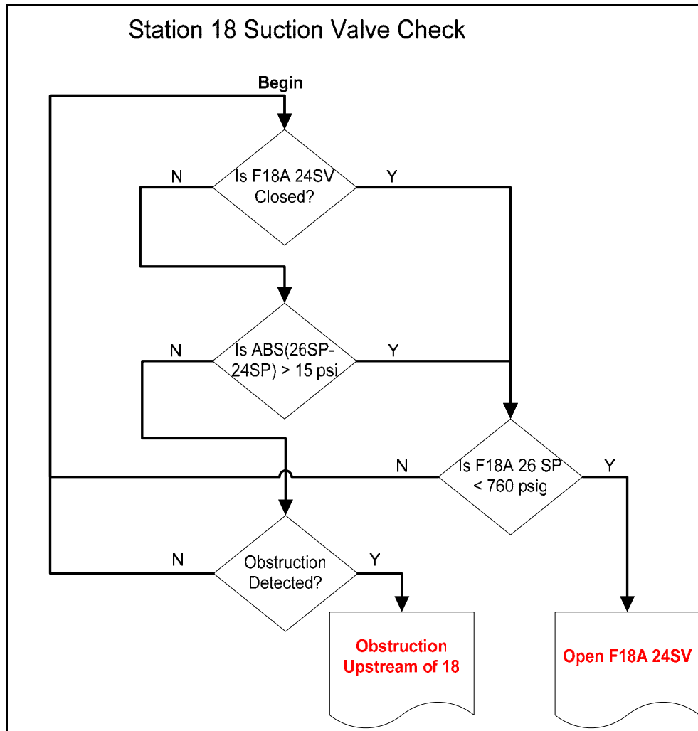
Figure 9. Station 18 suction valve alarm
