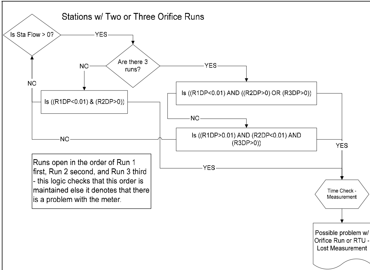
Figure 8. Meter station alarm
