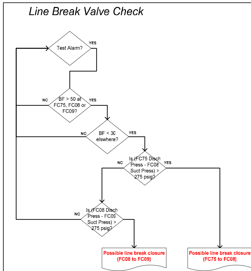
Figure 4. Line break operator alarm
