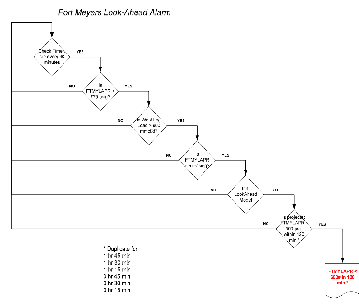
Figure 5. Fort Myers delivery pressure alarm
