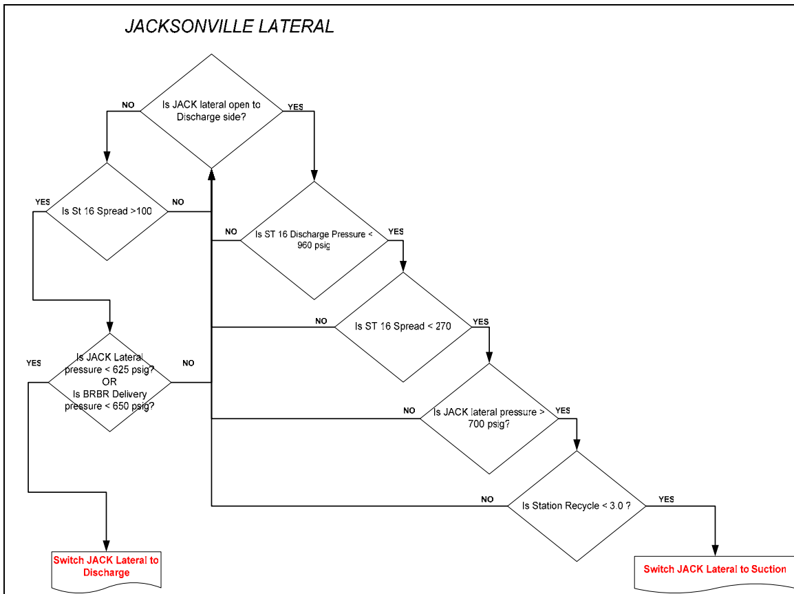
Figure 6. Jacksonville suction/discharge switch alarm
